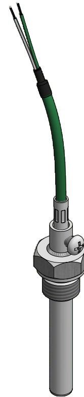
TTE150 Version with additional thermowell TSL cable insulation (teflon®FEP/silicone)
