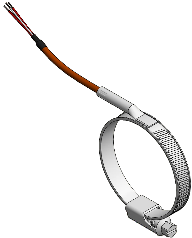
TOPE50244S TSL cable insulation (teflon®FEP/silicone)
