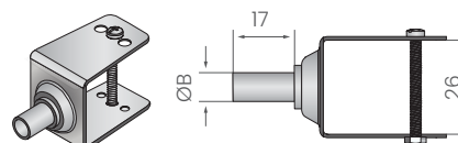
S-UB adaptor
