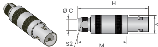
Lemo plug connector
