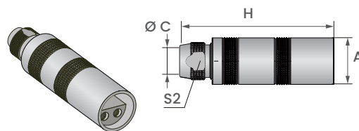
Lemo socket connector
